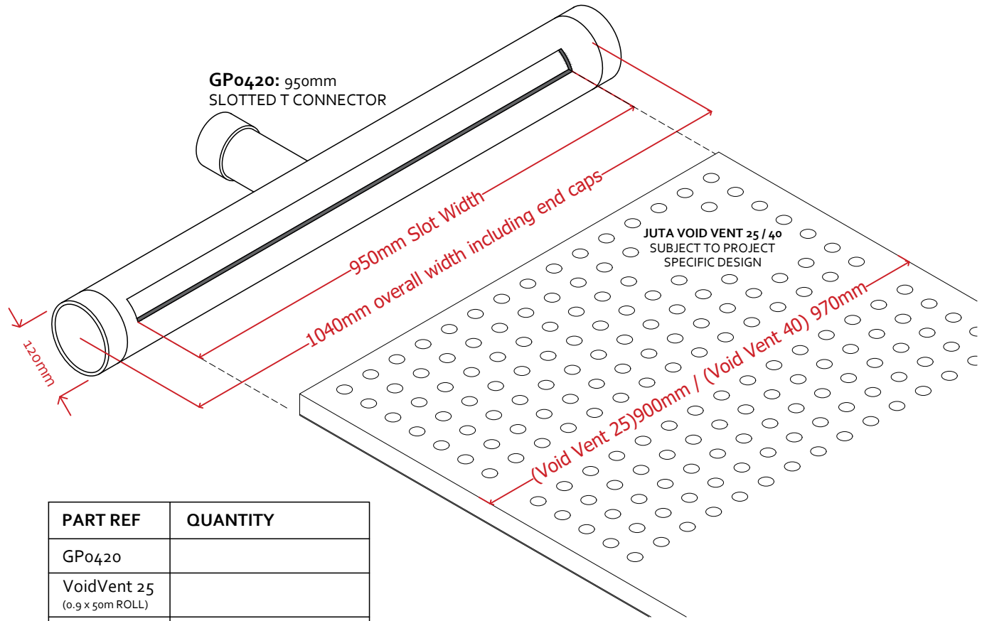
JUTA VOID VENT 25 / 40 SUBJECT TO PROJECT SPECIFIC DESIGN
